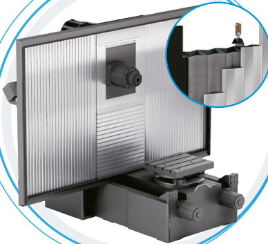
SCUDI X-Y CON SOFFIETTI X-Y SHIELDS WITH BELLOWS
