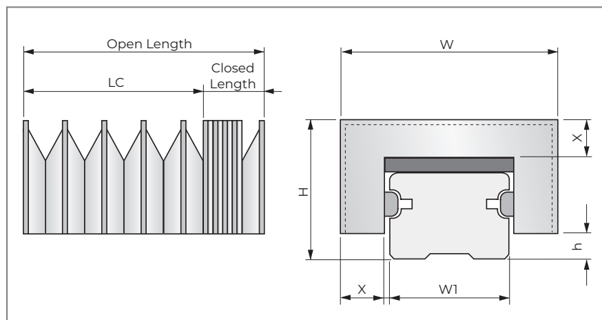
Example of bellows mounted on linear slides
